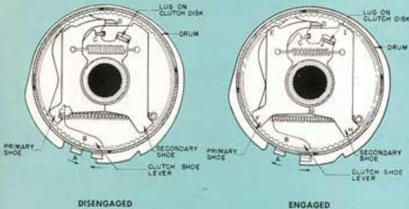
NEW CLUTCH DESIGN USES INTERNAL EXPANSION PRINCIPLE.
