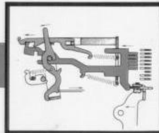
C Function reset bail forces function bar and engaged pawl to rear. Pawl engages function lever . . . function lever initiates operation of function.
