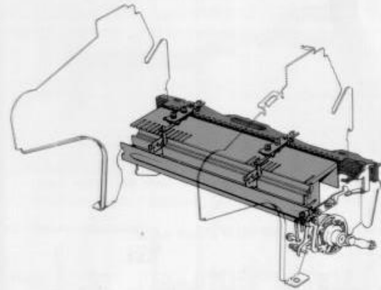
Partial section of typing unit in perspective shows stunt box in red and code bars in green. The two fork-like projections on top of the stunt box are called "shift forks." Shift forks position Suppression, Zero, and Figures—Letters Shift code bars through studs.
