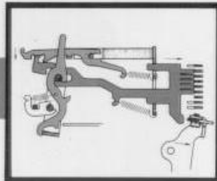
B If function bar tines find opening, function bar moves completely forward . . . function bar upper rear projection is engaged by falling function pawl.
