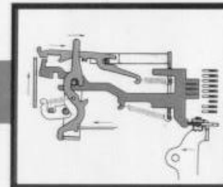
D Stripper blade removes pawl from function bar.
